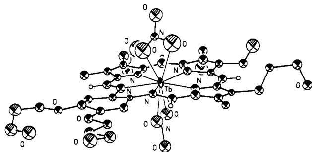
Figure 8. View of [\text{Tb-6}\cdot(\text{NO}_3)_2] showing the in-plane nature of the nine-coordinate metal center. Except for the Tb(III) atom, the structure was refined isotropically. Thermal ellipsoids are scaled to the 20% probability level.
