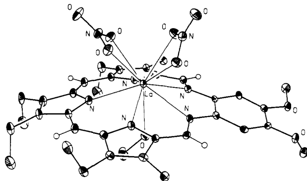
Figure 6. View of [La·3-MeOH·(NO 3 ) 2 ] showing the 10-coordinate nature of the complex. The metal center is 0.914 Å above the mean-square pentaaza plane.
