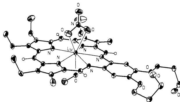
Figure 5. View of [Lu·5-MeOH·NO 3 ] + showing the eight-coordinate nature of the complex. The metal center is 0.269 Å above the mean-square pentaaza plane.
