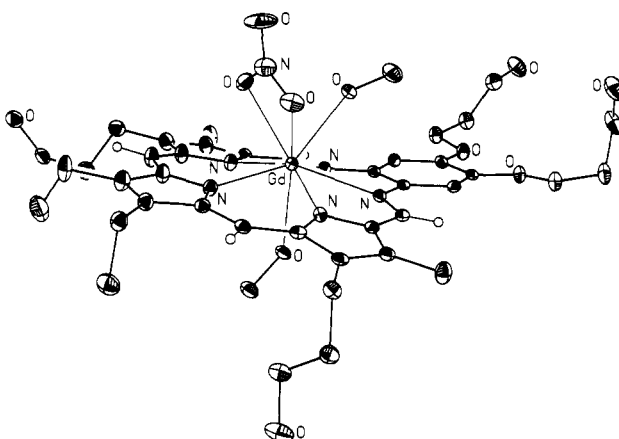
Figure 7. View of [Gd·6-(MeOH) 2 ·NO 3 ] + showing the nine-coordinate nature of the complex. The metal center is 0.595 Å above the mean-square pentaaza plane.
